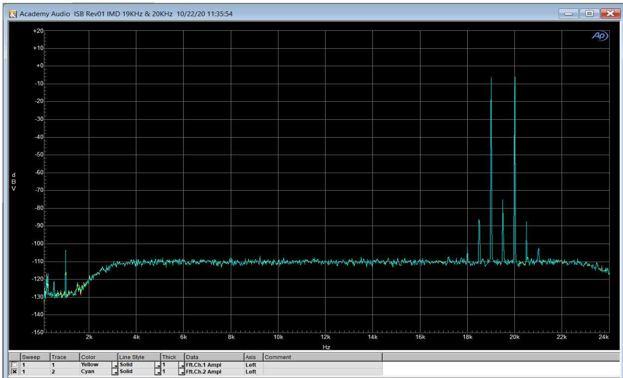
Figure 4. IMD 19KHz and 20kHz spectrum.
