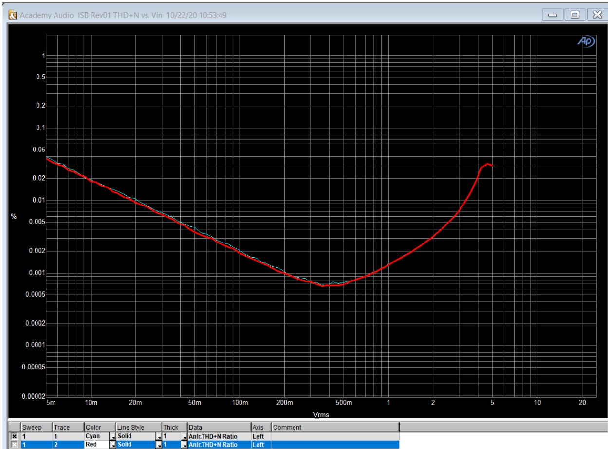
Figure 1. THD+N vs. Vin
