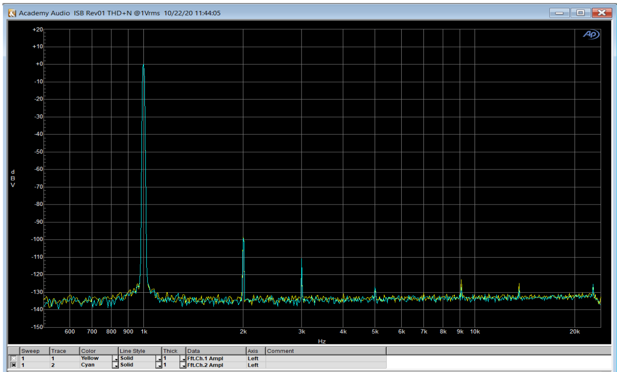
Figure 2. THD+N Spectrum.
