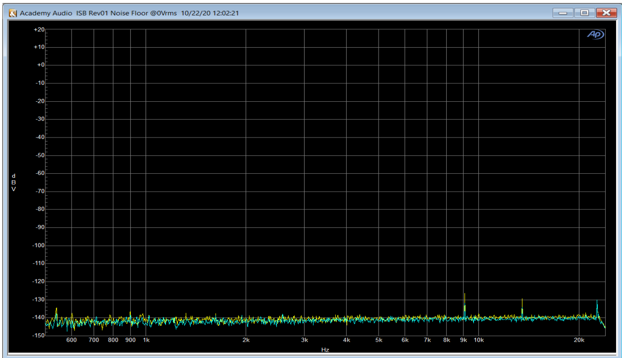
Figure 5. Noise Floor Spectrum with LPS9 Power Supply. Noise Level = -109dBV (3.6uV)
