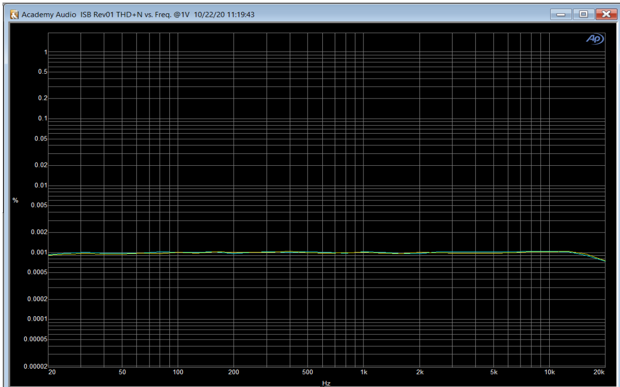
Figure 3. THD+N vs Frequency @1Vrms.
